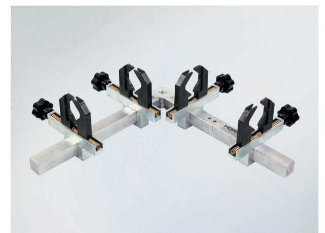
Component positioner
